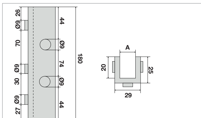
Pattino L.180 SCHINDLER
